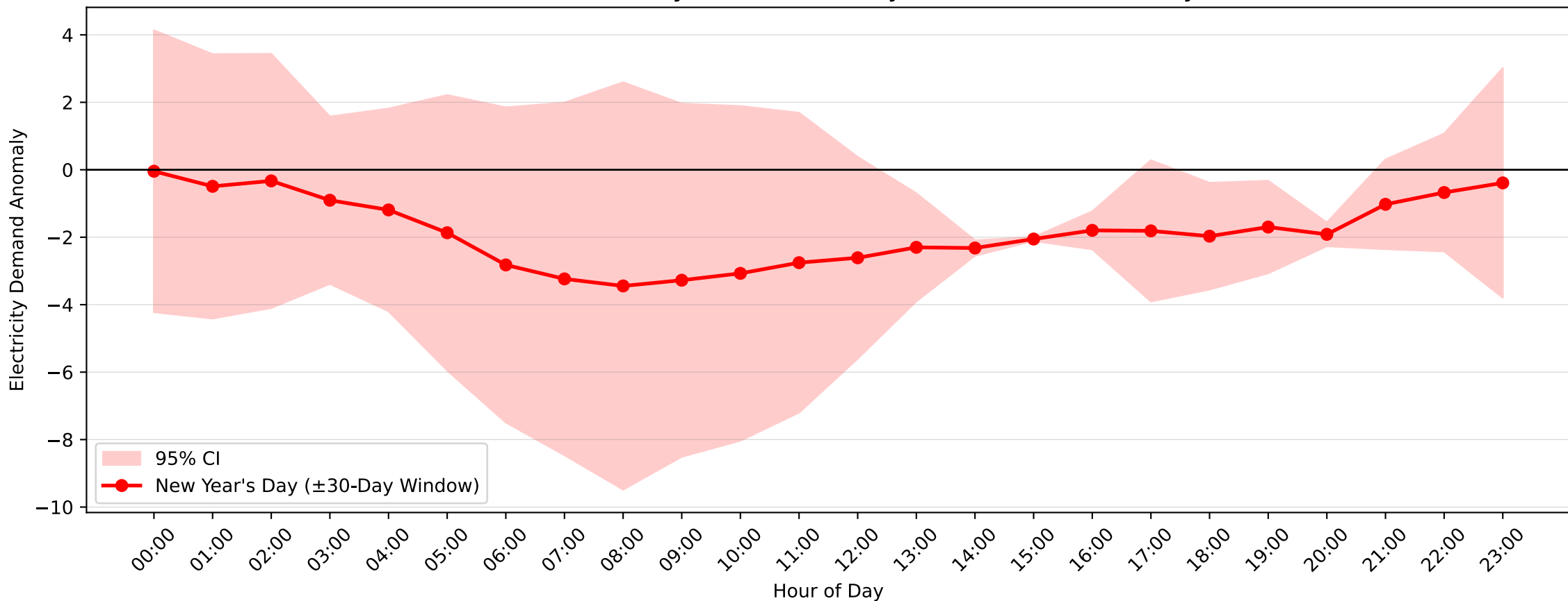
Bass Hill Demand Anomaly: New Year's Day (2004-2005, \pm 30 -Day Window)
